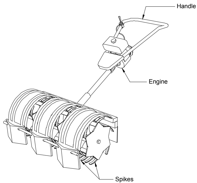
Figure 7 – Power-Weeder
