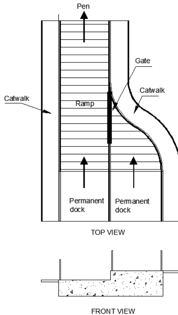
Figure 2 – Permanent multilayer dock with ramp
