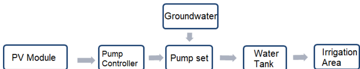
Figure 3. Configuration setup for a groundwater source with reservoir
