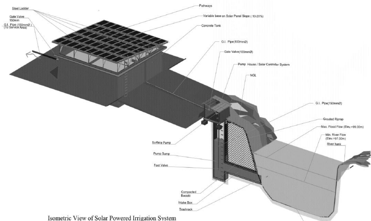
Figure 5. Example of an SPIS
